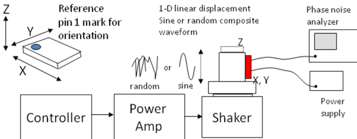
Figure 1. Sinusoidal and random vibration test setup
