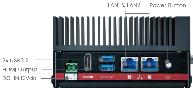
Front I/O
